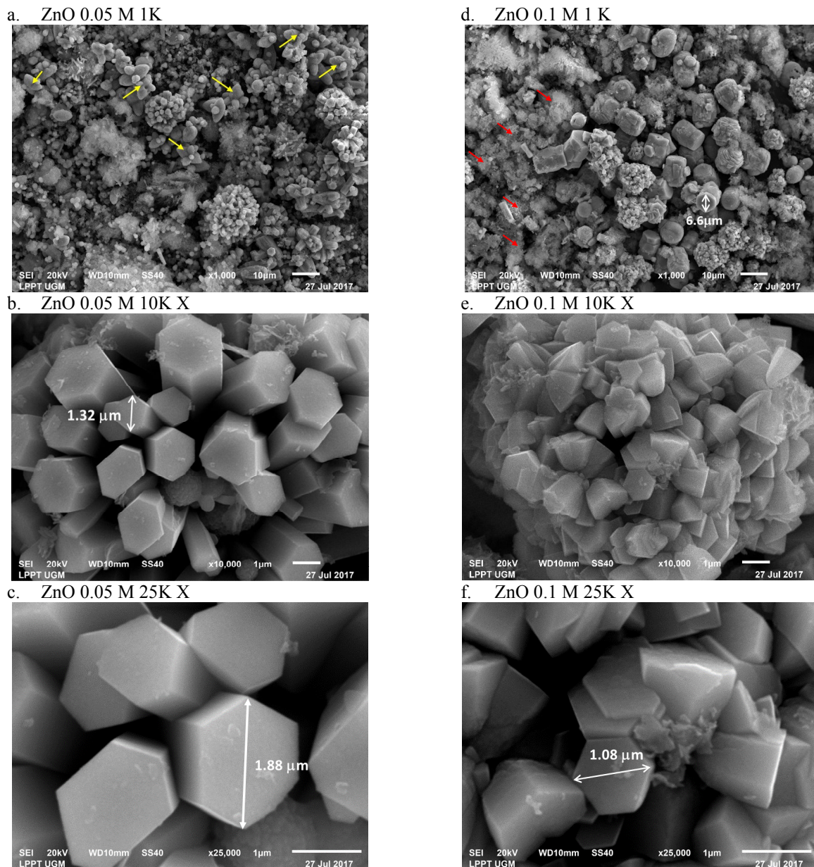
Figure 2. SEM Results of ZnO Micro-Nanorod Structures Synthesized at Concentration of 0.05 and 0.1 M
